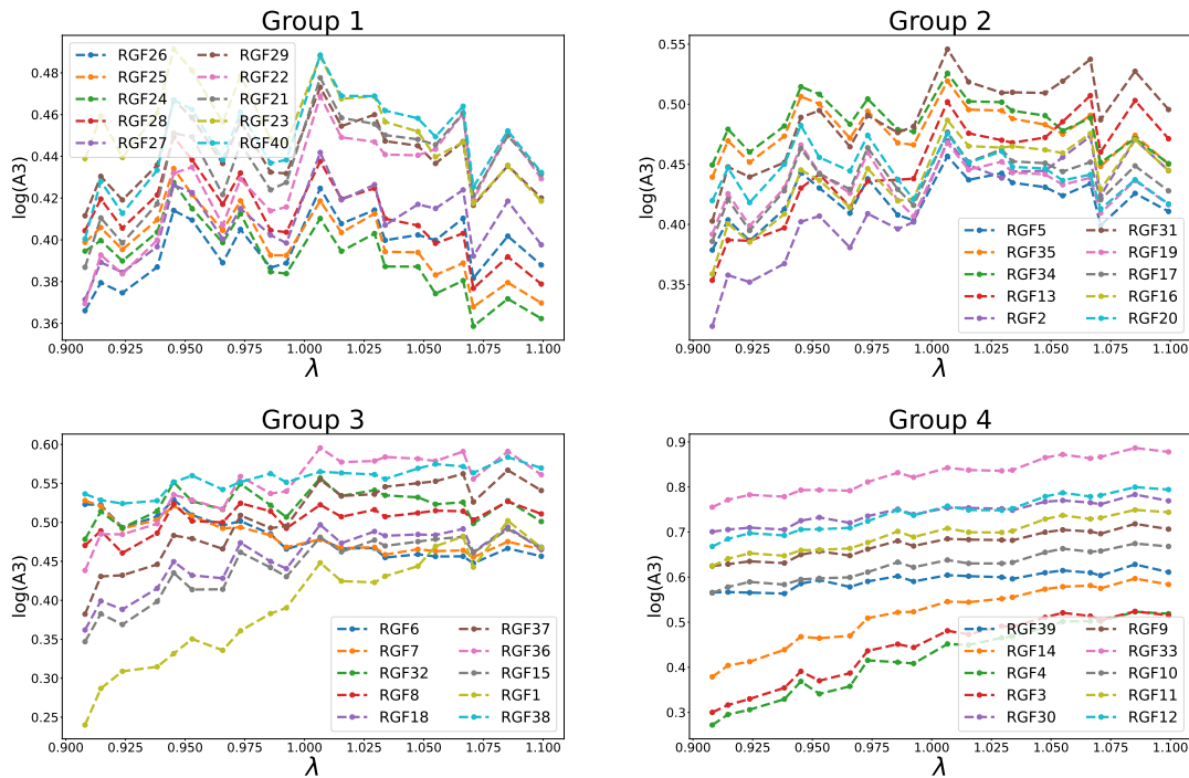
Figure 4.15: Plots of coefficient g_{\lambda_k,1}(\mathbf{x}_i) associated with \log(\theta_3) estimated for i = 1, \dots, n = 40 as a function of \lambda_k with k = 1, \dots, m = 20 .
