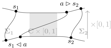
Figure 5.4: The skein category of the gluing is balanced
