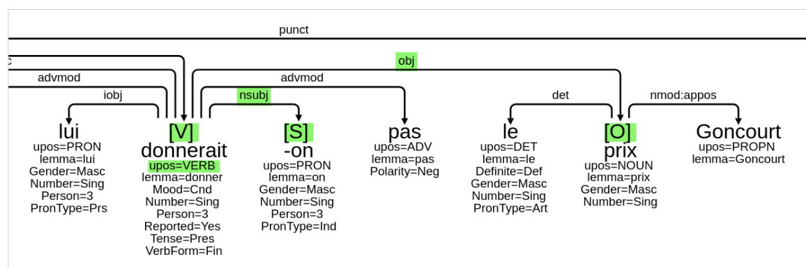
Figure 1.4: Top: screenshot illustrating a query for a VSO pattern using the Grew-Match tool [Guillaume, 2021]. Below: The only two sentences (in red) found in the French Rhapsodie Treebank for VSO with their corresponding dependency trees. Both examples are of interrogative form, known for allowing an SV order swap. S, V and O are highlighted in green.
