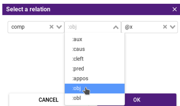
Figure 5.3: Interface for the relation selection for a SUD project configuration.
