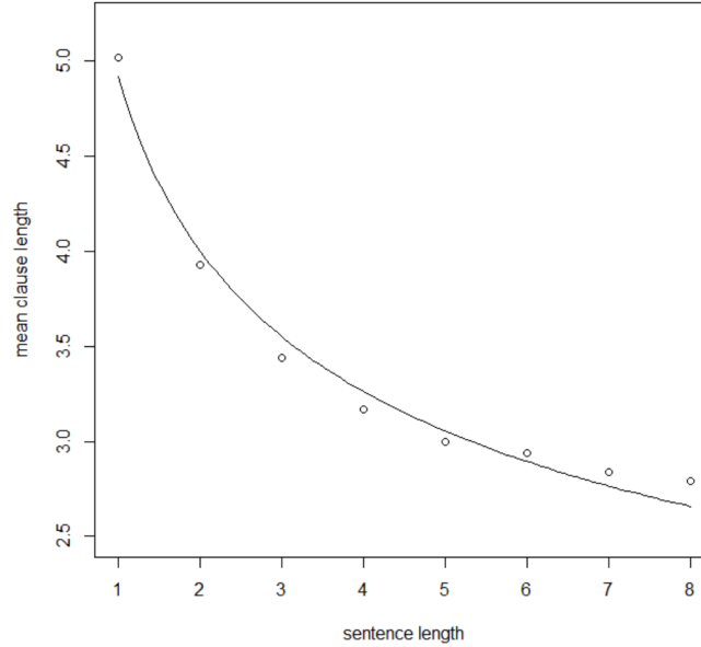
Figure 6.5: The MAL modelled by function y(x) = ax^b as the relation between sentence length and the mean clause length
