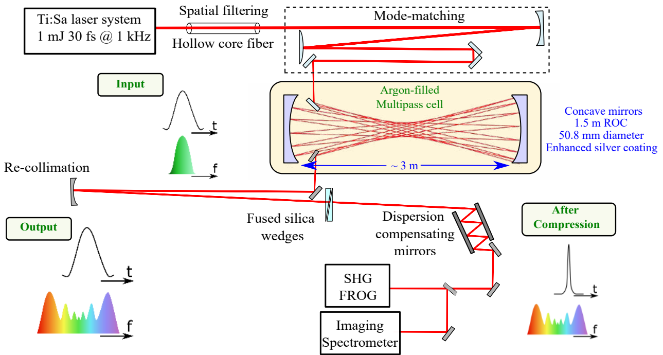
Figure 3.4: A schematic layout of the MPC-based post-compression setup. For clarity, only a few passes in the MPC are represented.
