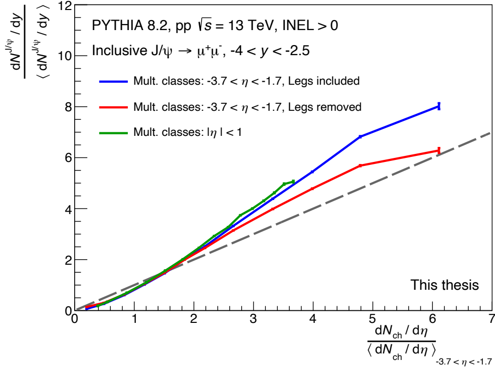
Figure 3.16: J/ψ relative yield as a function of the relative multiplicity in the V0C acceptance -3.7 < \eta < -1.7 obtained with PYTHIA 8.2 simulations with including or excluding the J/ψ daughters from the multiplicity estimation, and with a different multiplicity selection based on the number of charged particles in |\eta| < 1 .
