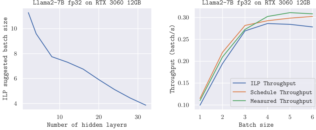
Figure 4.8: Batch size selection of Llama2-7B. Left: for models with different layers, suggested batch size value (continuous) from O-ILP. Right: For 32-layer model, throughput (batch/time) using fixed batch sizes.
