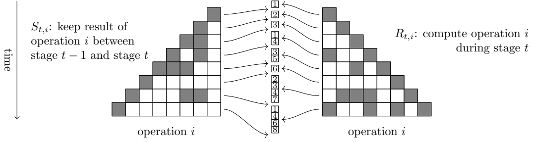
Figure 2.1: Visualization of CHECKMATE formulation where the middle columns shows a sequence of operations being (re)computed in order, and its representation in ILP variables is showed on the right. The left side shows when the tensor are saved in memory.
