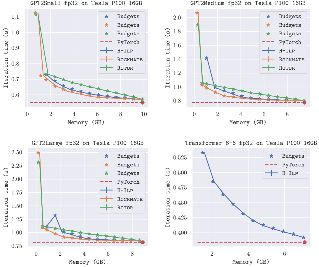
Figure 3.13: Experiments on sequential networks: ROCKMATE are tailored for those models, as discussed in Chapter 2.
