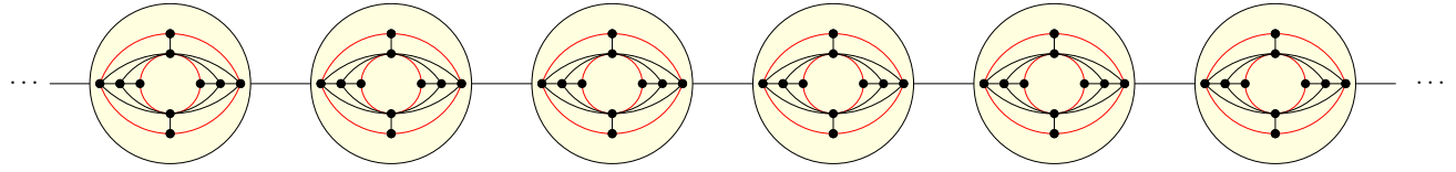
Figure 1.3: The path-decomposition of the graph from Figure 1.2 obtained after applying theorem 3.7 to the nested family of red cycles. The red cycles form the adhesion sets of the path-decomposition.
