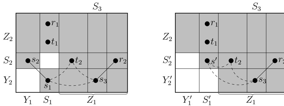
Figure 1.6: Left: The graph G when S_2 is incident to exactly 2 crossed edges. Here t_2 is part of no crossed edge and S_2 and S_3 are crossing via the crossed edge r_2s_3 . Hence, \text{fc}(S_2) = \{s_1, t_2, s_3\} . Right: The graph G' obtained after contracting the crossed edge s_1s_2 . The dashed edges are edges that appear in H and H' respectively. The situation is identical when S_2 is incident to 3 crossed edges, but harder to illustrate in 2 dimensions.
