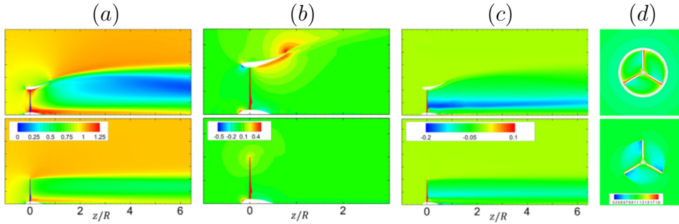
Figure 8.6: Comparison between the ducted (DAWT) (Top) and open (OWT) (Bottom) configurations for V_\infty = 7 \text{ m/s} : (a) azimuthally-averaged normalized axial velocity, (b) azimuthally-averaged normalized radial velocity contours, (c) azimuthally-averaged normalized tangential velocity contours, (d) normalized axial velocity contours at the rotor plane. Figure adapted from Bontempo and Di Marzo [2023]
