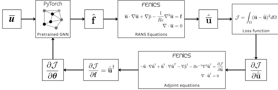
Figure 7.1: End-to-end training loop; \bar{\mathbf{u}} is the GNN's input mean flow; \hat{\mathbf{f}} is the GNN's predicted forcing stress term; \theta are the GNN's trainable parameters; \mathcal{J}(\hat{\mathbf{u}}) is the cost function to minimize.
