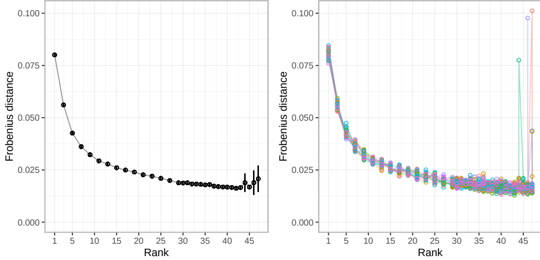
Figure 4.13: Cross-validation results for the tensor decomposition. Left: Frobenius distance mean of the 30-fold cross-validation with a confidence interval at 95% around each point with the rank varying between 1 and 47. Right: Frobenius distance for each of the 30 folds. The rank of the decomposition is chosen by taking the lowest rank (here 41) contained in the confidence interval from the rank minimizing the error (here 43).
