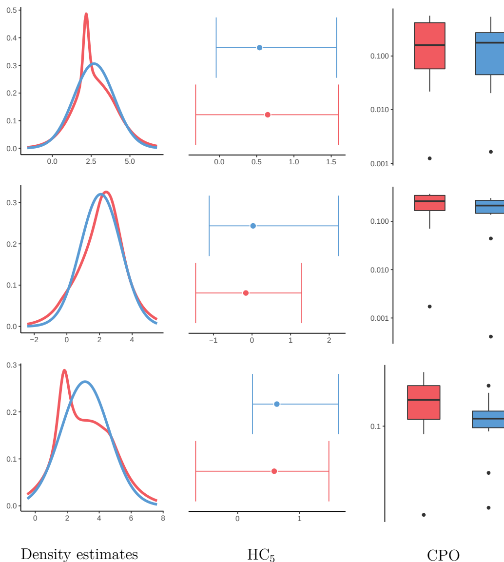
Figure 4.12: Density estimates, HC_5 and CPO for three small censored datasets. Red (—) for the BNP model, blue (—) for the normal model (KDE not implemented for censored data). From top to bottom: Phosmet, Naled, Sodium dichromate.
