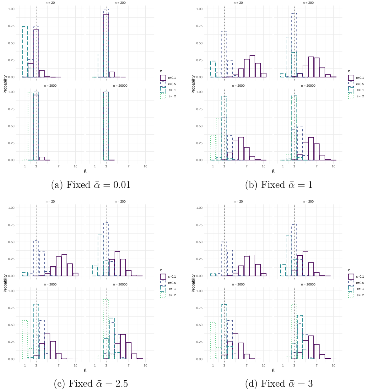
Figure 2.5: Distribution of \tilde{K} , that is the posterior number of clusters after applying the Merge-Truncate-Merge algorithm of Guha et al. (2021) , with c parameter in \{0.1, 0.5, 1, 2\} , under a Dirichlet multinomial process mixture with fixed parameter K = 10 , and various choices of \bar{\alpha} = \alpha/K and n .
