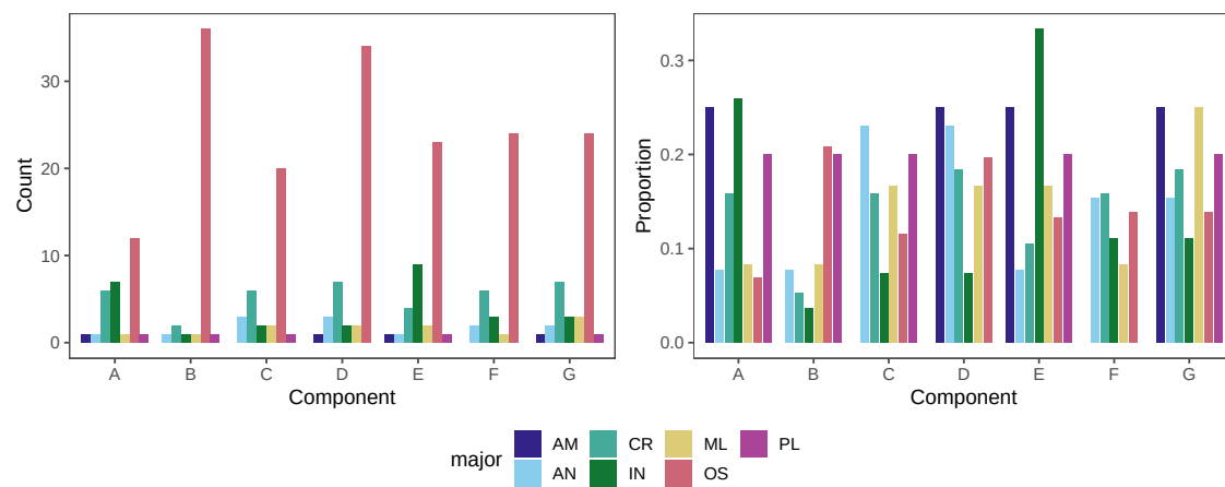
Figure 4.19: Taxonomic composition of the selected components at the major level.
