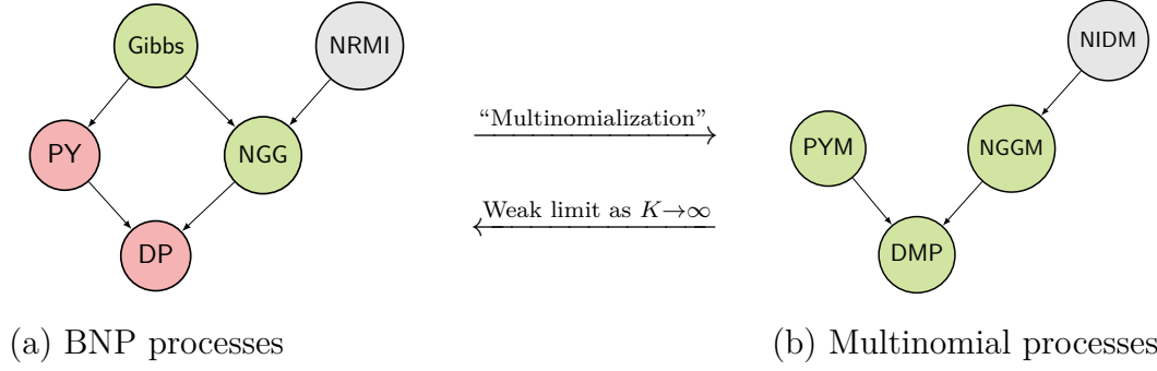
Figure 2.1: Graphical representation of the relationships between the discrete mixing measures considered in this article. An arrow indicates that the target is a special case of the origin. (a) BNP processes: Gibbs-type priors (Gibbs), normalized random measures with independent increments (NRMI), Pitman–Yor process (PY), normalized generalized Gamma process (NGG), and Dirichlet process (DP). (b) Multinomial processes (finite-dimensional approximations of their respective BNP counterparts in the left panel): normalized infinitely divisible multinomial process (NIDM), Pitman–Yor multinomial process (PYM), normalized generalized Gamma multinomial process (NGGM), Dirichlet multinomial process (DMP). Going from left to right can be done according to a “multinomialization” of the BNP processes as described in Section 2.2.3, while the reverse direction is achieved by taking a weak limit as K \rightarrow \infty . Our contributions generalize results known for mixing measures in red to mixing measures in green. The case of mixing measures in gray remains an open problem.
